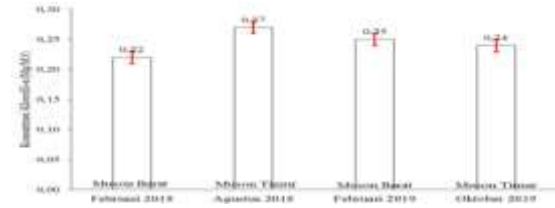
Figure 2. Average value of chlorophyll-a concentration hanintyo algorithm in Birah-birahan Island waters for 2 years
