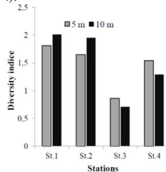
Figure 4. Index of biodiversity genus coral in Pulau Miang in all depths
